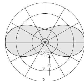
Typical Horizontal Pattern
